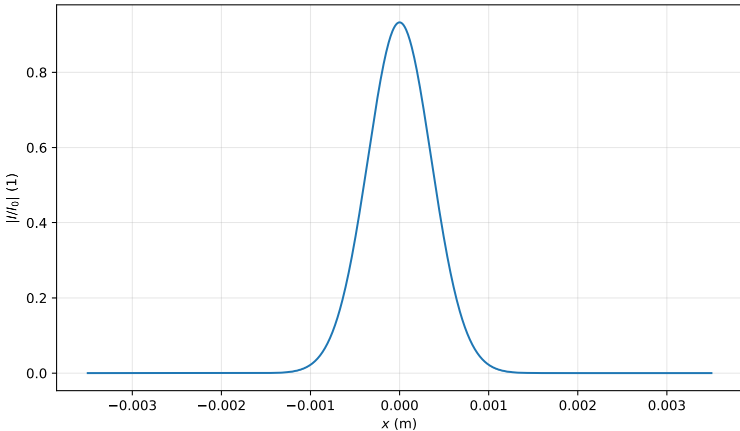
Intensity profile I(x, y = 0, z = 0.637m)/I_0 , P_{in}=0.1P_{cr} , artificial time
